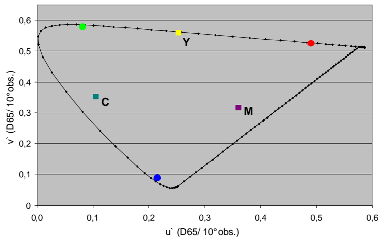
Resulting ( u^*/v^* )- color coordinates for a light source D65 (under AOI 0°)
