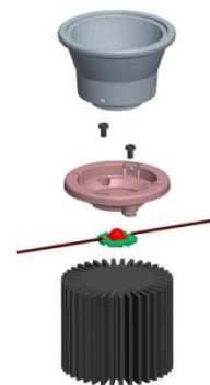
Example for mounting the reflector
