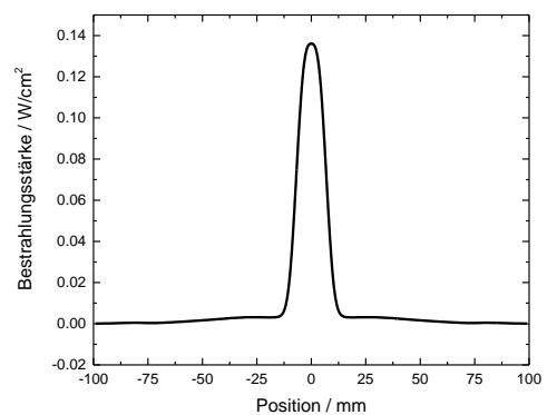
Near field distribution in 100 mm distance with 1 W LED power
